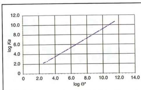
Figure 1. Kármán number as a function of Q^* for smooth pipe ( \epsilon = 0 ).
